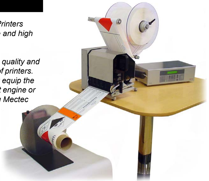
T70 Desktop version together with an external label rewinder.
